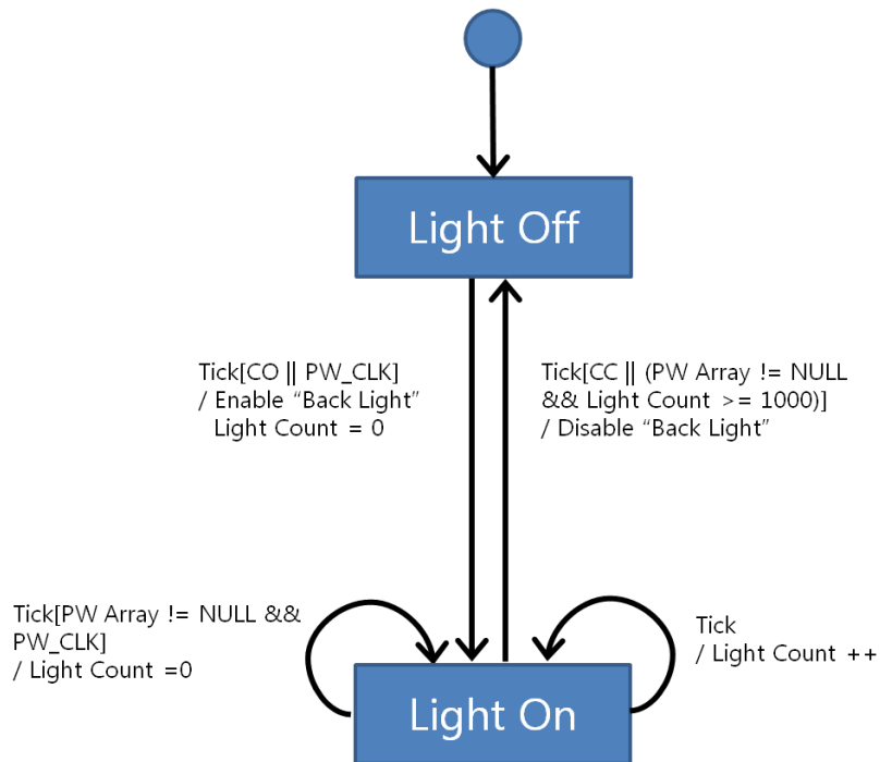
3.2.4.4.4 State Transition Diagram for Light Controller(2.2.2)
