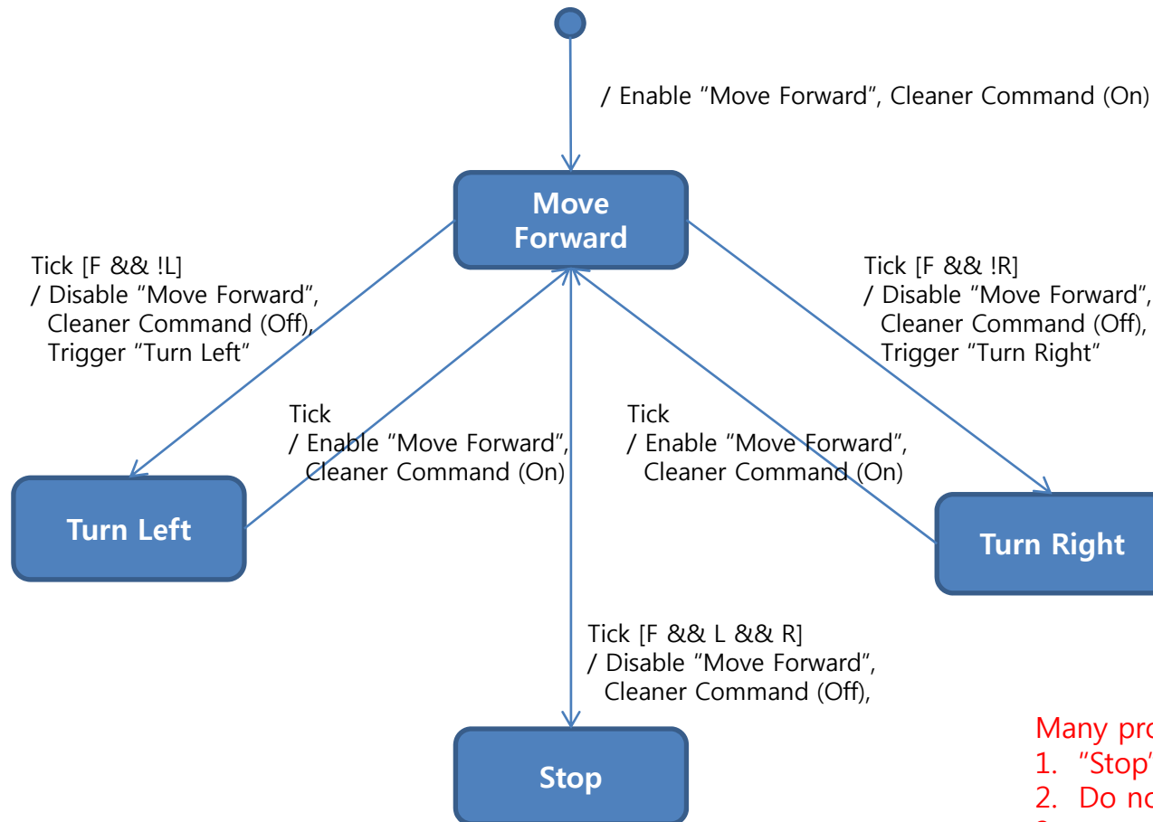
State Transition Diagram for Controller 2.1.1
