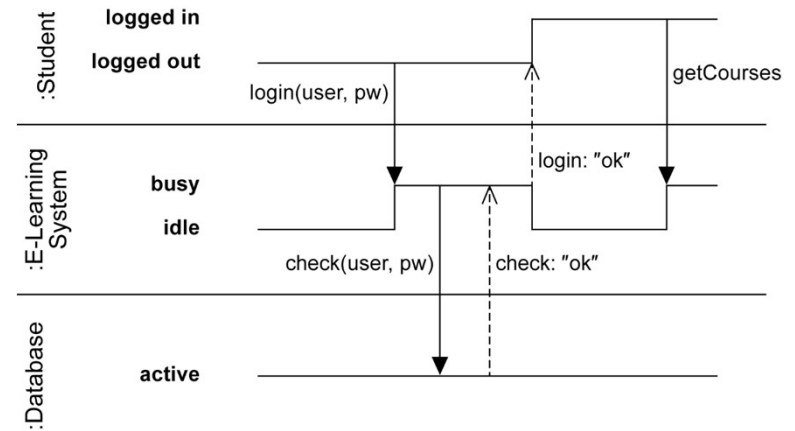
Timing diagram
