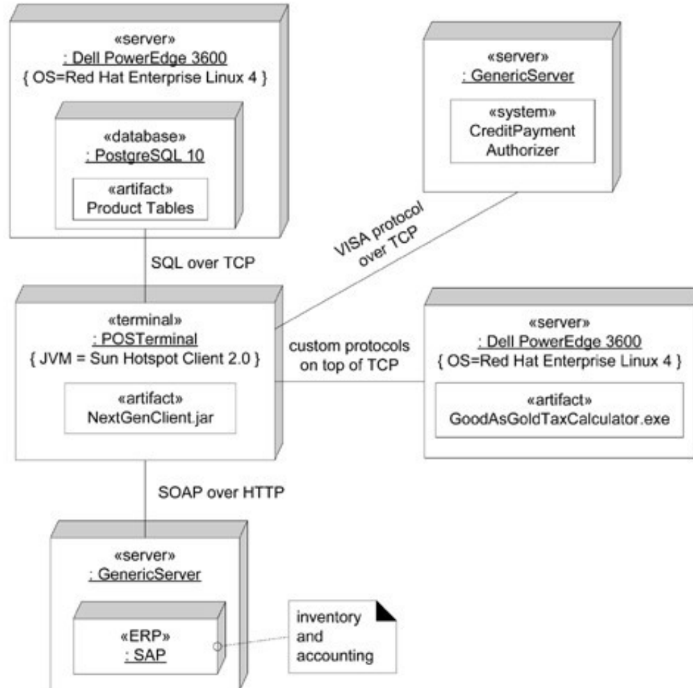
Deployment View
