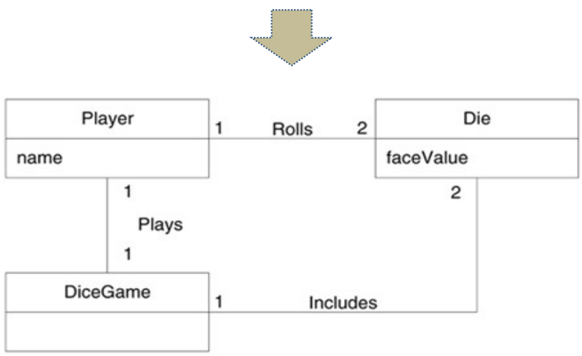
Domain Model
