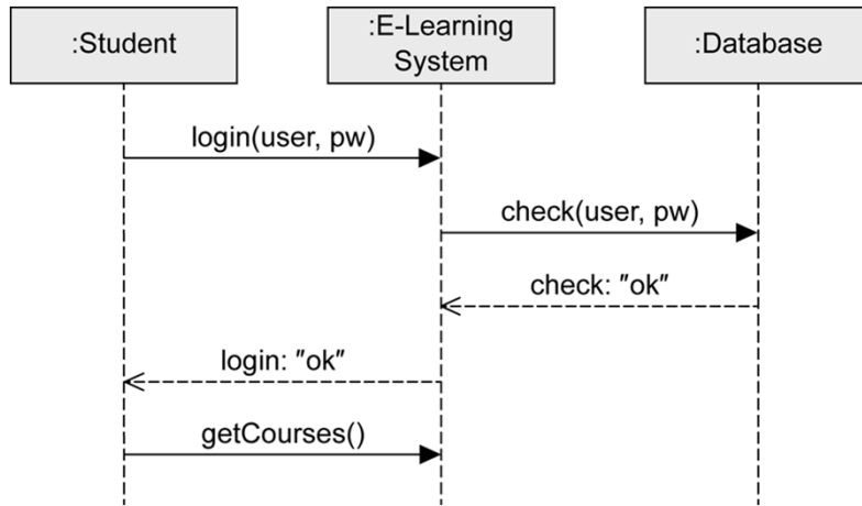
Sequence diagram
