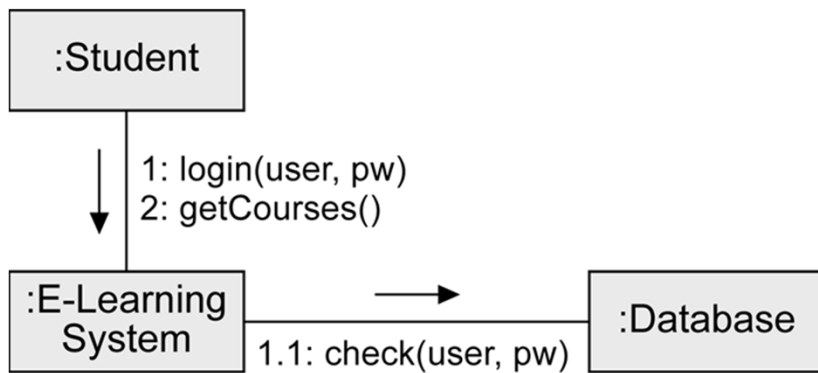
Communication diagram
