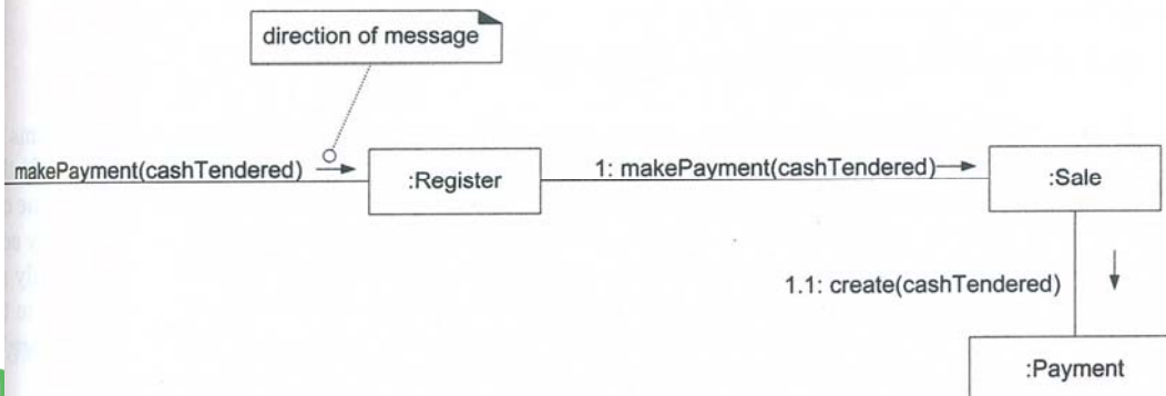
Example Communication Diagram: makePayment
