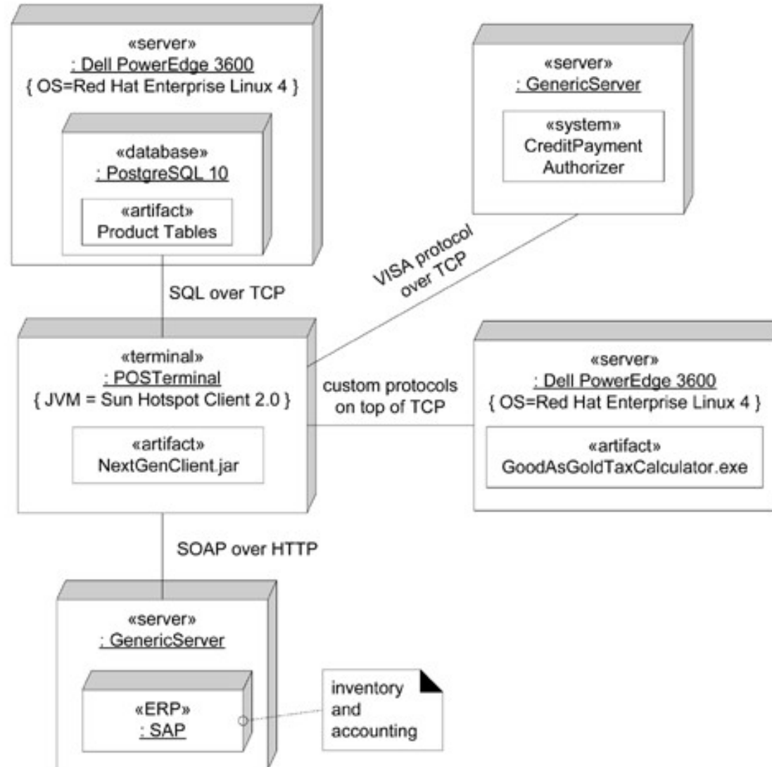
Deployment View
