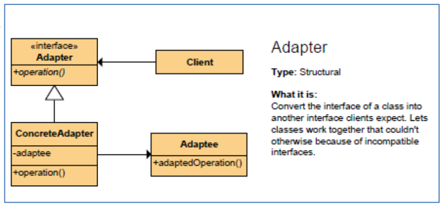
Design Pattern of GoF
