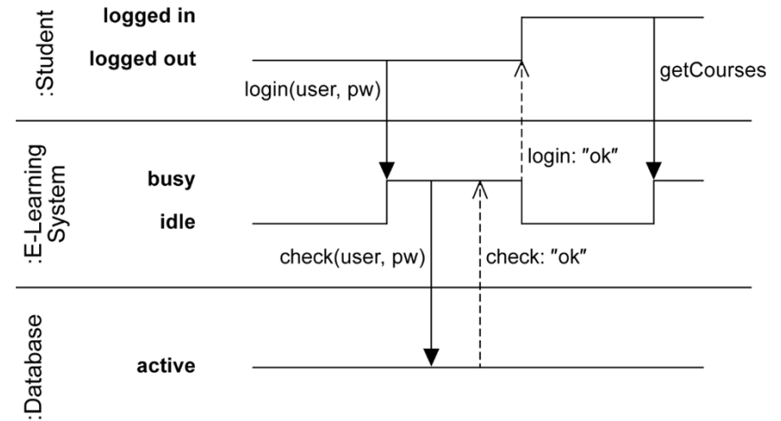
Timing diagram
