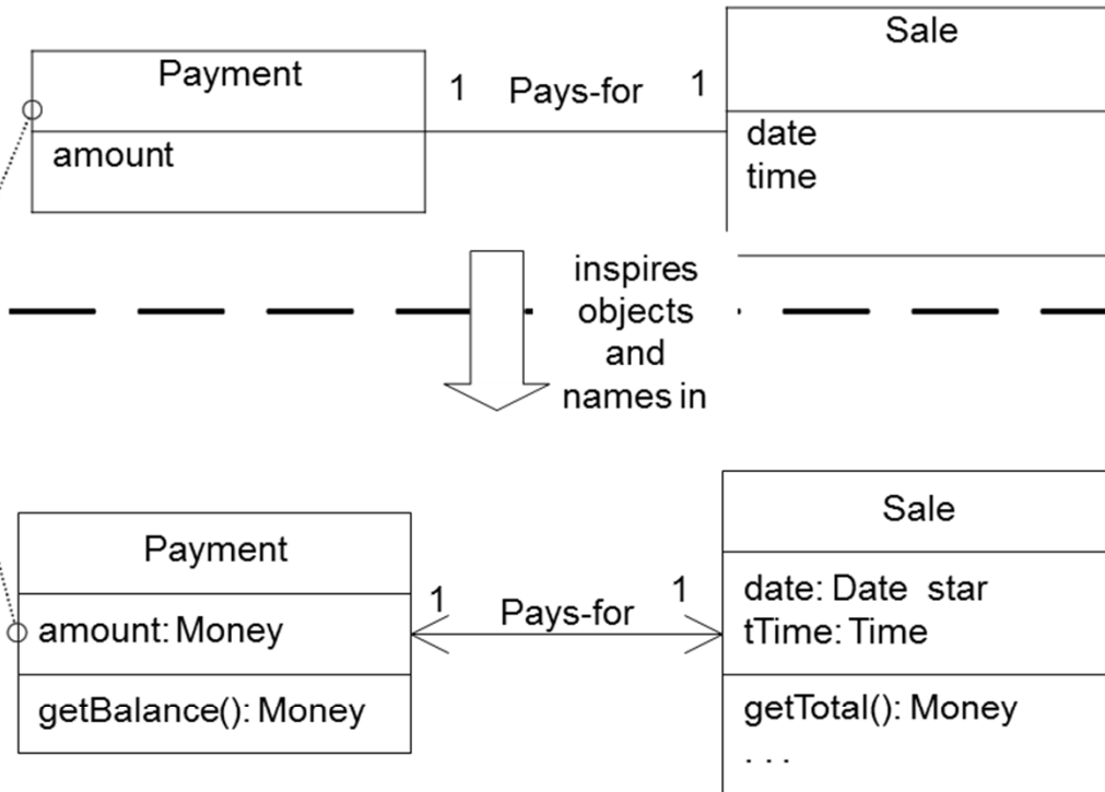
UP Domain Model Stakeholder's view of the noteworthy concepts in the domain.
