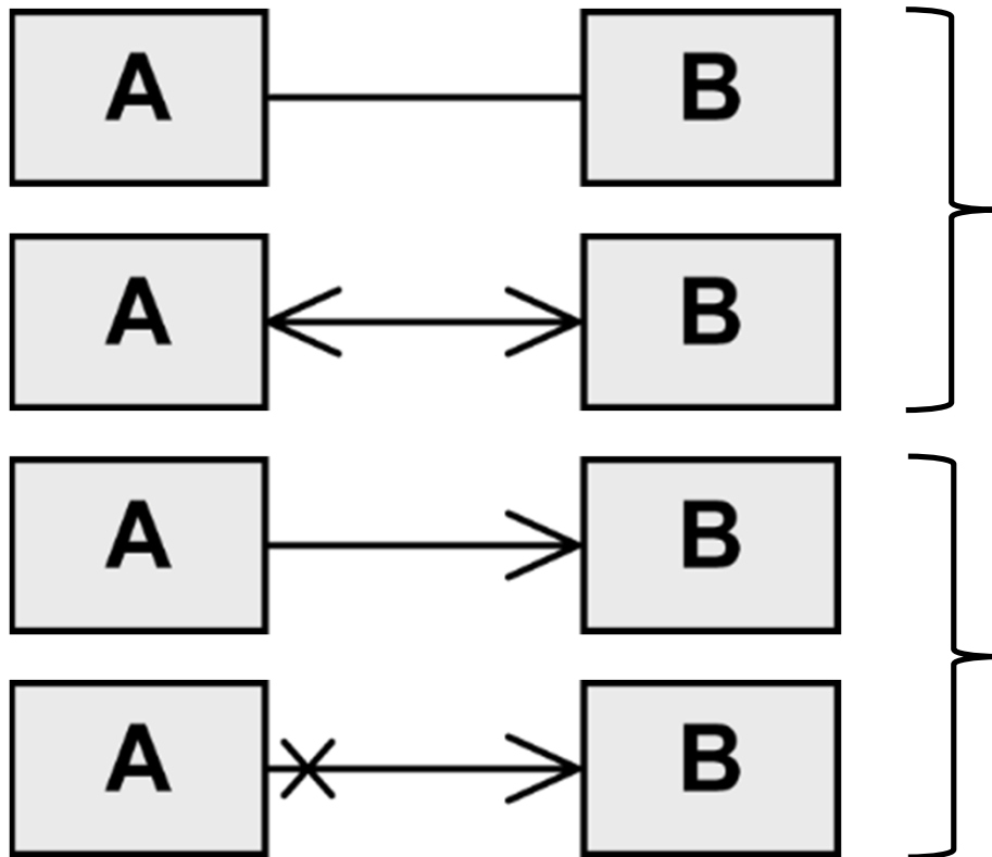
UML Standard
