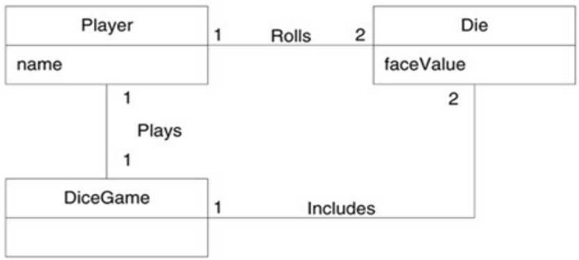
Domain Model
