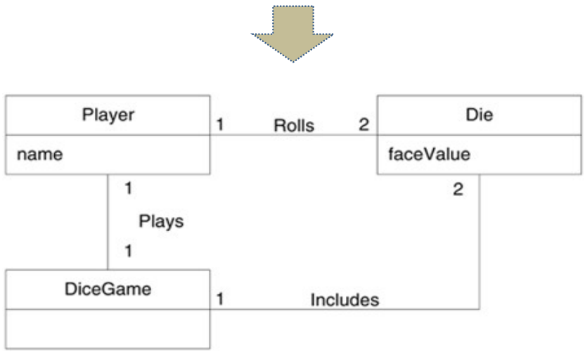
Domain Model
