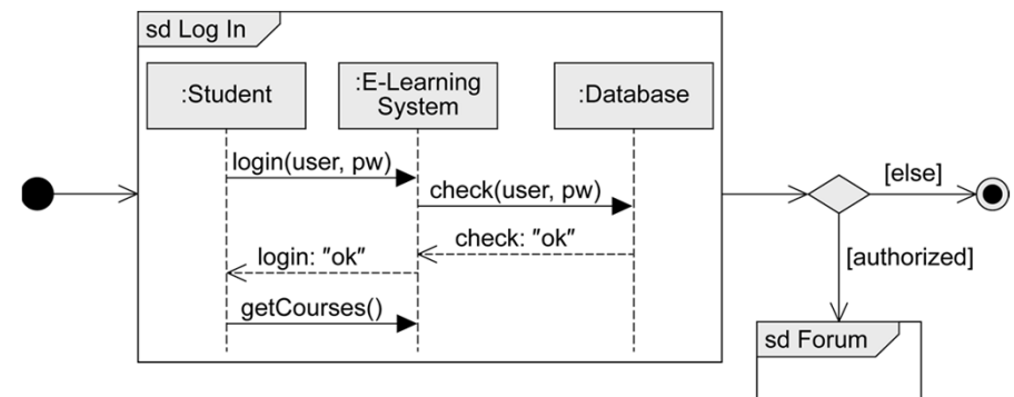
Interaction Overview diagram
