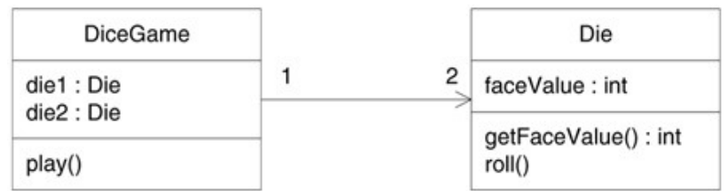
Design Class Diagram
