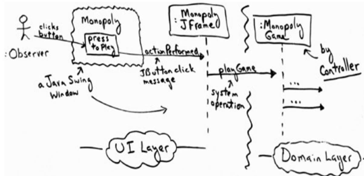
Applying the Controller pattern using MonopolyGame . Connecting the UI layer to the domain layer of software objects.
