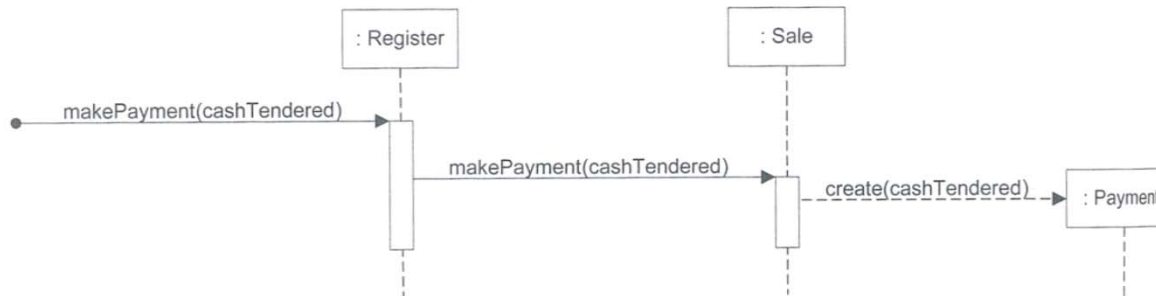
Example Sequence Diagram: makePayment
