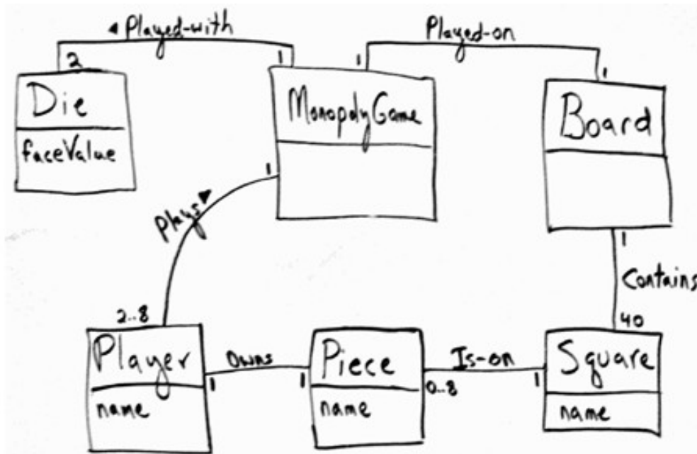
Monopoly iteration-1 domain model
