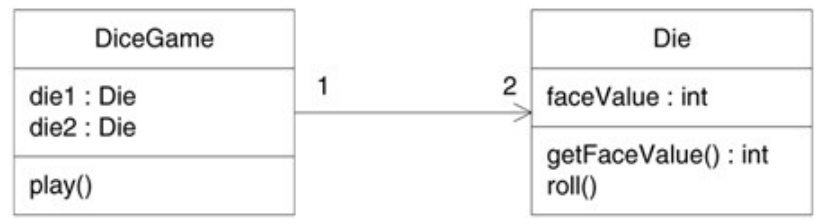
Design Class Diagram
